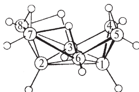
(12) B_8H_{12}
