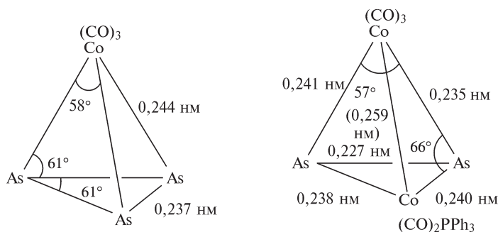
Рис. 13.22. Строение комплексов [\text{As}_3\text{Co}(\text{CO})_3] и [\text{As}_2\{\text{Co}(\text{CO})_3\}\{\text{Co}(\text{CO})_2(\text{PPh}_3)\}]
