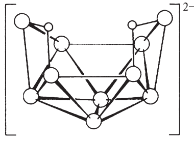
(38) B_{10}H_{12}^{2-}
