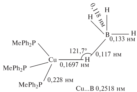
а [\text{Cu}^{\text{I}}(\eta^1\text{-BH}_4)(\text{PMePh}_2)_3]
