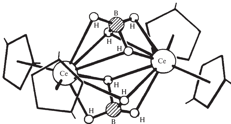
e \text{ [Ce}(\mu:\eta^4\text{-BH}_4)(\eta^5\text{-C}_5\text{H}_3\text{Bu}'_2)_2
