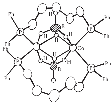
d \text{ [Co}(\mu:\eta^3\text{-BH}_4)_2\{(\mu\text{-Ph}_2\text{P}(\text{CH}_2)_5\text{PPh}_2)\}_2
